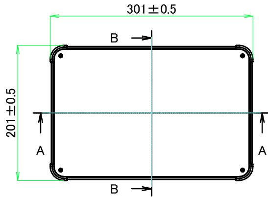
E view
